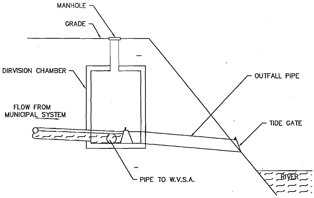
NORMAL OPERATION
